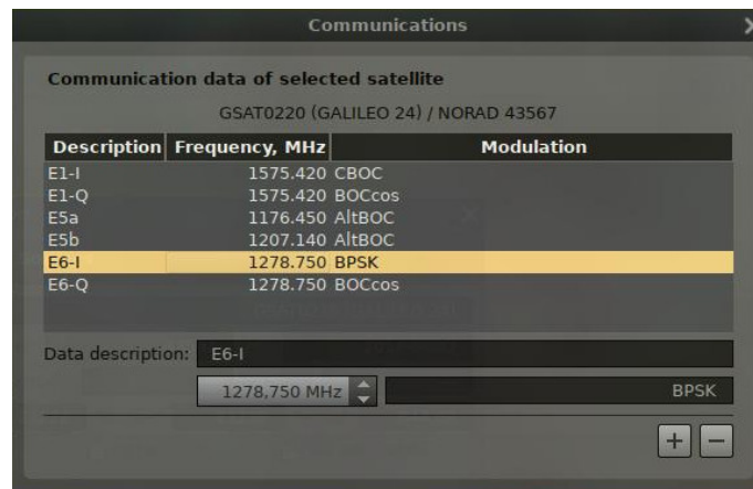
Figure 14.14: Configuration of the Satellites plugin: satellite communication data
