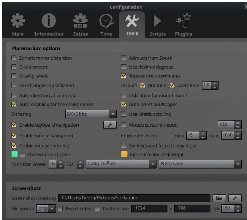
Figure 4.7: Configuration Window: Tools Tab
