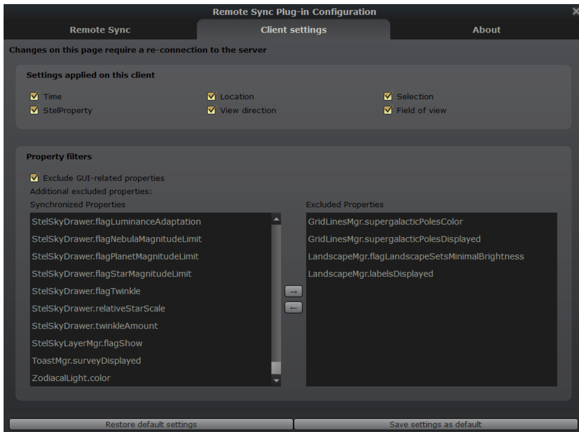
Figure 13.6: RemoteSync client settings window
