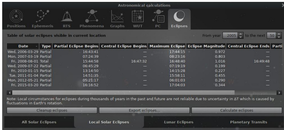
Figure 4.43: Astronomical Calculations (AstroCalc): Eclipses / Local Solar Eclipses
