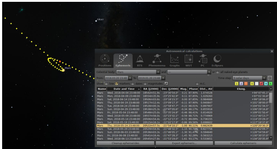
Figure 4.26: Astronomical Calculations (AstroCalc): Plot trace of planet
