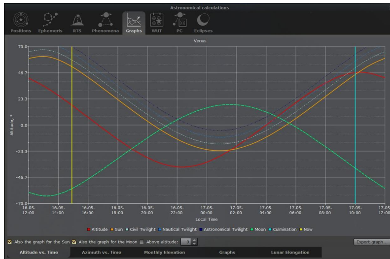
Figure 4.33: Astronomical Calculations (AstroCalc): Graphs / Altitude vs. Time
