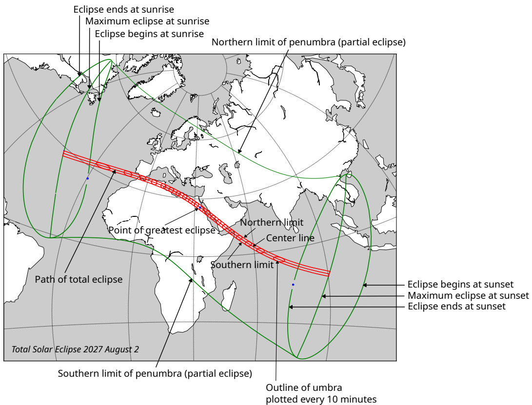
Figure 4.42: Key to solar eclipse map
