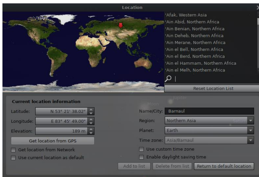
Figure 4.2: Location window
