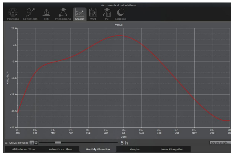
Figure 4.35: Astronomical Calculations (AstroCalc): Graphs / Monthly Elevation
