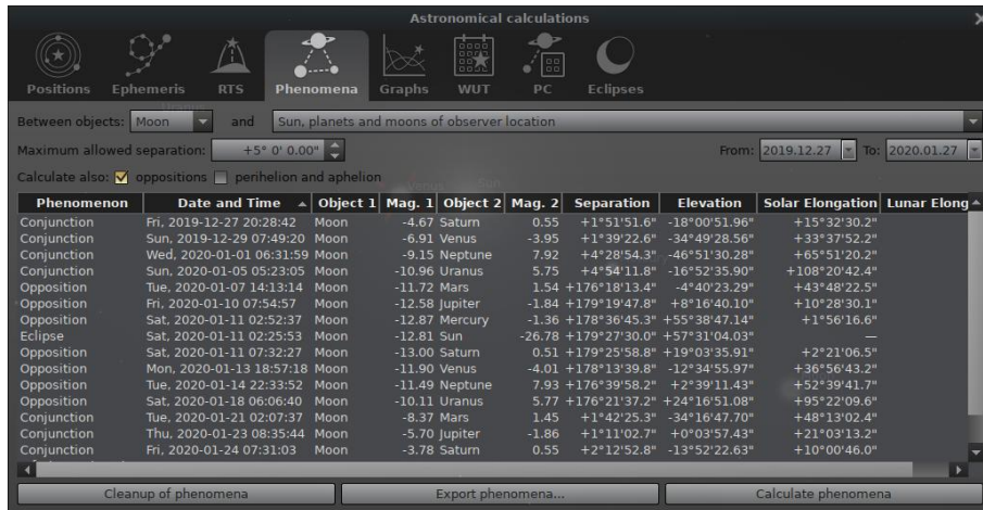
Figure 4.32: Astronomical Calculations (AstroCalc): Phenomena
