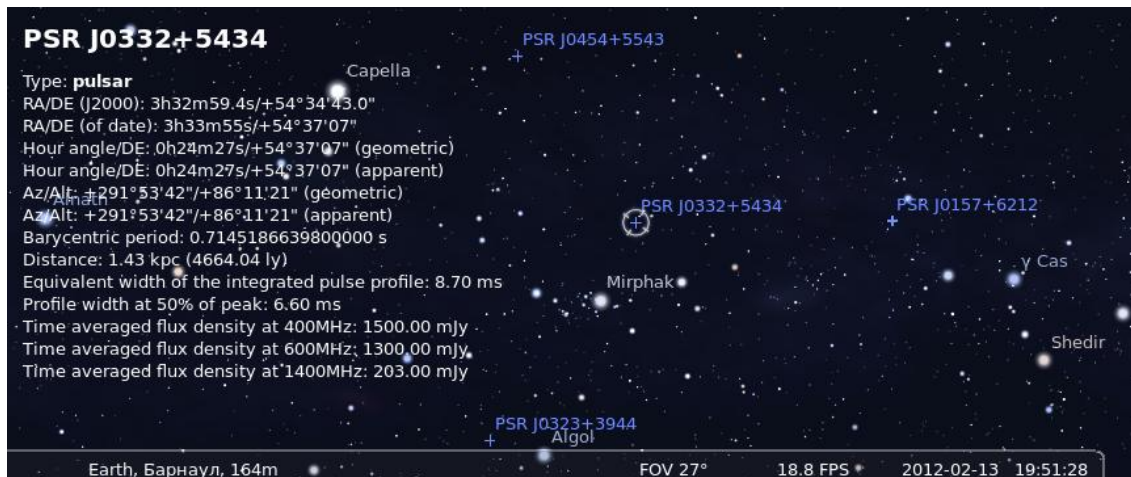
Figure 14.5: PSR J0332+5434
