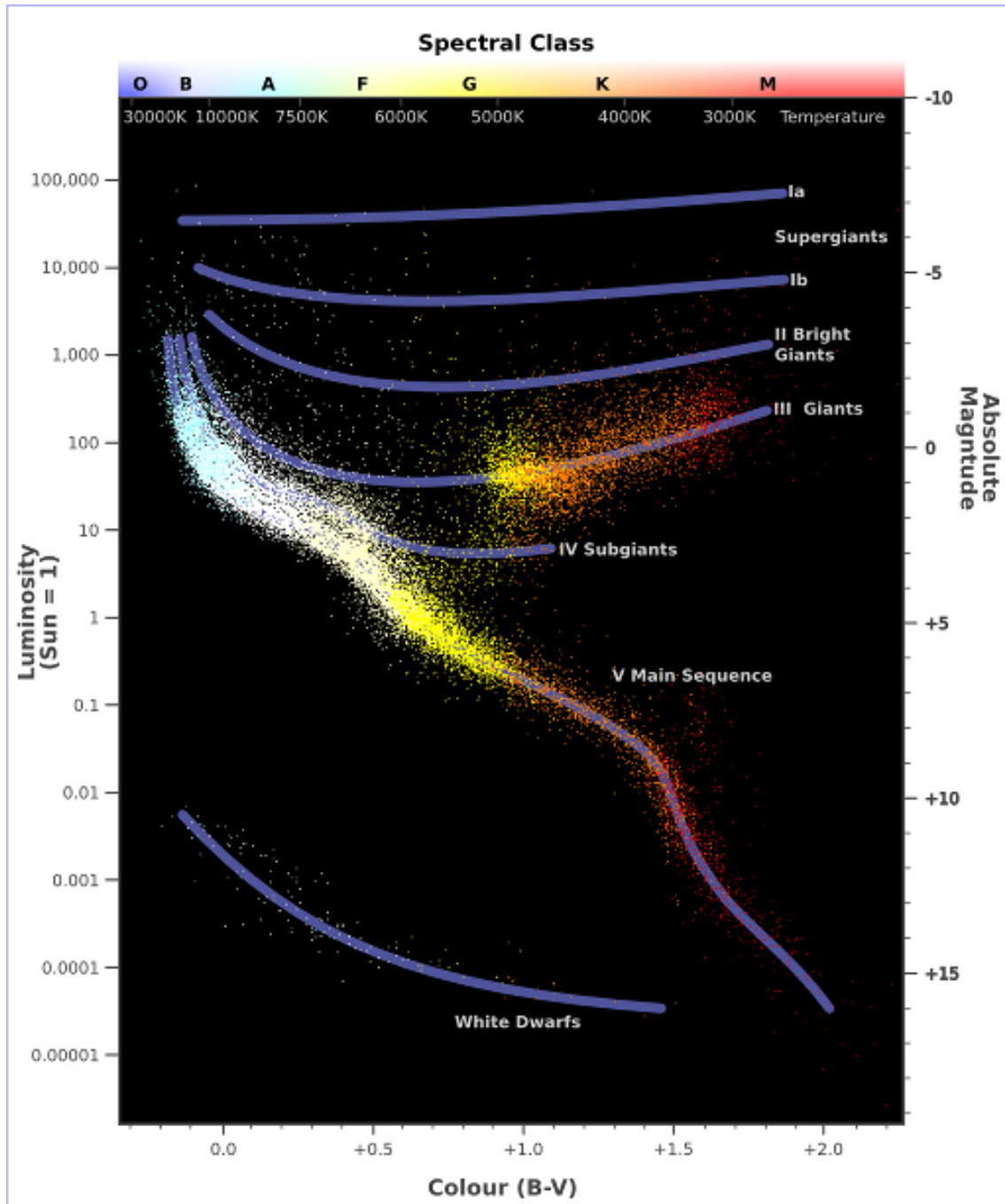
Figure 19.3: Hertzsprung-Russell Diagram
