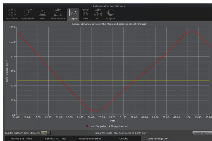
Figure 4.37: Astronomical Calculations (AstroCalc): Graphs / Lunar Elongation
