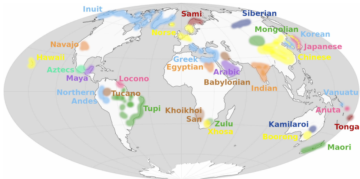
Figure 4.15: World map showing Stellarium’s built-in set of sky cultures. To avoid overcrowding, smaller European sky cultures which are mostly derivatives or relatives of the “Modern” sky culture are not shown. (Image: S. M. Hoffmann)
