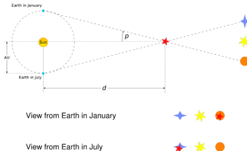
Figure 18.7: Stellar Parallax
