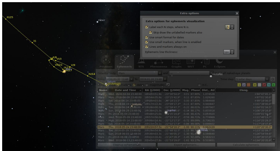
Figure 4.27: Astronomical Calculations (AstroCalc): Extra options for ephemeris
