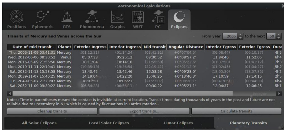
Figure 4.45: Astronomical Calculations (AstroCalc): Eclipses / Planetary Transits
