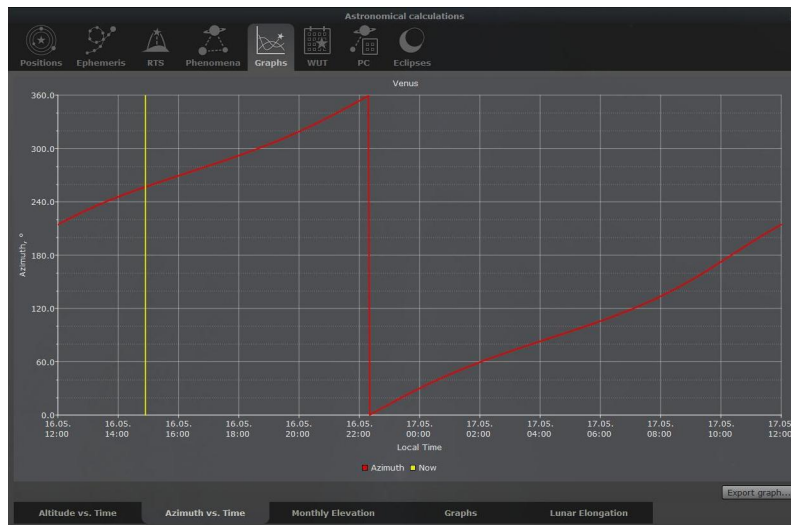
Figure 4.34: Astronomical Calculations (AstroCalc): Graphs / Azimuth vs. Time
