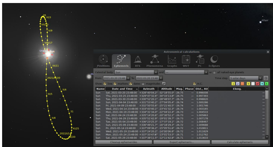
Figure 4.28: Astronomical Calculations (AstroCalc): Analemma on the Earth
