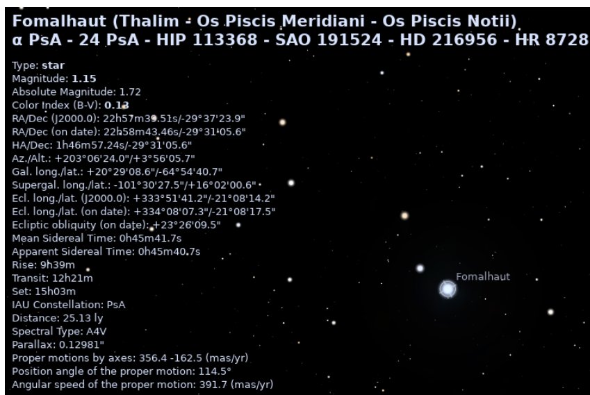
Figure 19.2: Star Names and Data
