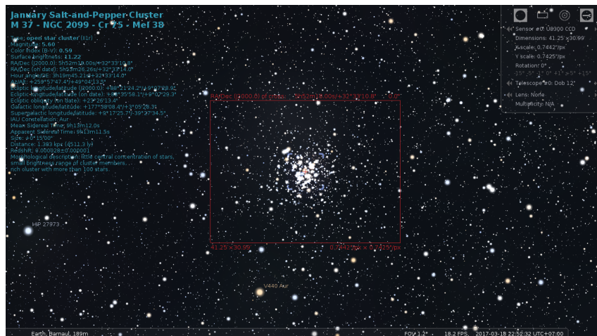
Figure 16.3: View of M37 through a CCD sensor of the Oculars plugin.
