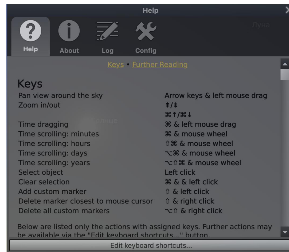
Figure 4.46: Help Window
