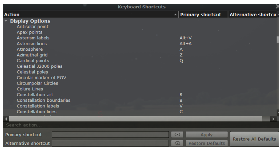
Figure 4.50: Keyboard Shortcuts
