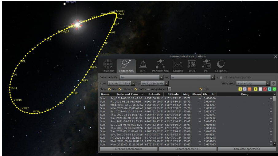
Figure 4.29: Astronomical Calculations (AstroCalc): Analemma on Mars
