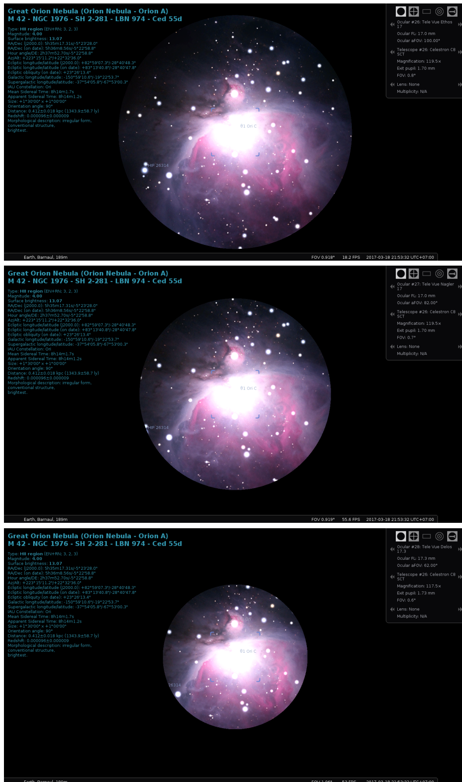
Figure 16.17: Comparing apparent fields of view of (top) a 17 mm Tele Vue Ethos eyepiece with an aFOV of 100°. Magnification is 119.5x. (center) a 17 mm Tele Vue Nagler eyepiece with an aFOV of 82°. Magnification is 119.5x. (bottom) a 17.3 mm Tele Vue Delos eyepiece with an aFOV of 62°. Magnification is 117.5x.
