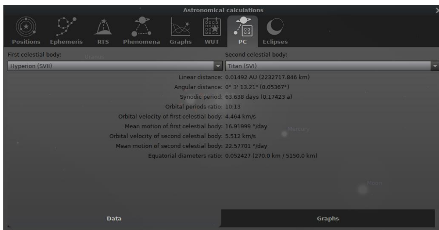
Figure 4.39: Astronomical Calculations (AstroCalc): Planetary Calculator (PC), Data Tab
