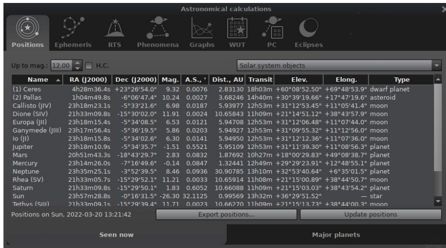
Figure 4.24: Astronomical Calculations (AstroCalc): Celestial positions / Seen now
