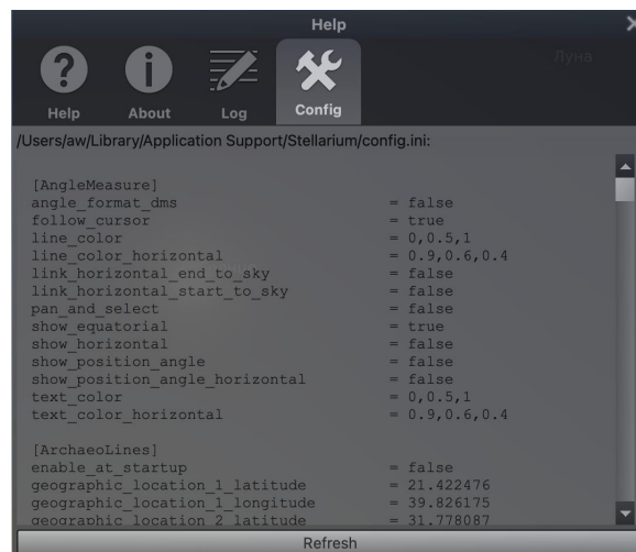
Figure 4.49: Help Window: Config file
