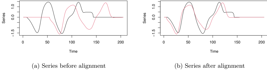
Figure 6: Visualization of the NCCc-based alignment performed on two sample series. After alignment, the second (red) series is either truncated and/or prepended/appended with zeros so that its length matches the first (black) series.
